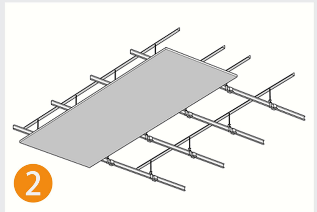
2 Install stainless steel honeycomb panels one by one along the triangular sub keel
