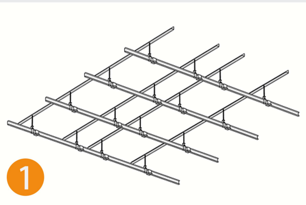
1 Install expansion screws, fix the screw rod and hook, install the main keel and triangular sub keel
